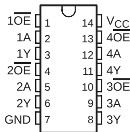
SN54LV125 . . . J OR W PACKAGE SN74LV125 . . . D, DB, OR PW PACKAGE (TOP VIEW)
