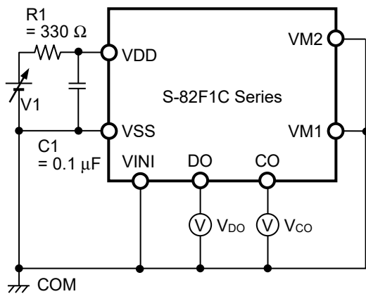
Figure 3 Test Circuit 1
