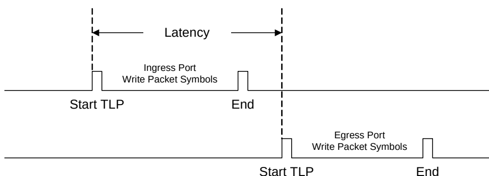
Figure 8-11. Start TLP-to-Start TLP Latency Measurement
