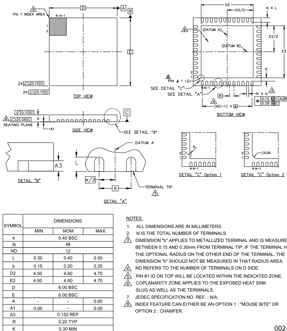
Figure 14 48L-QFN 6 mm × 6 mm × 0.6 mm package outline
