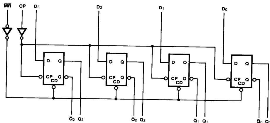
LOGIC DIAGRAM
