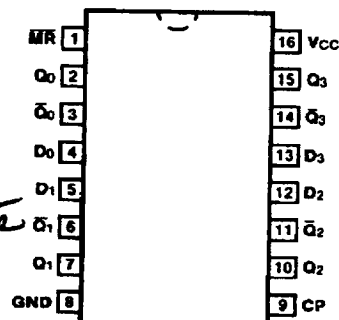
CONNECTION DIAGRAM PINOUT A
