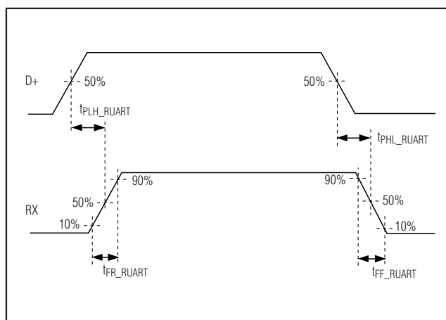
Figure 14. UART Receiver Timing
