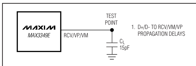
Figure 8. Test Circuit for Receiver Propagation Delay
