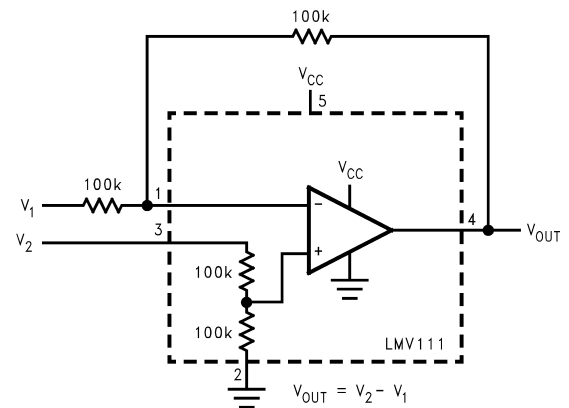
FIGURE 4. Difference Amplifier
