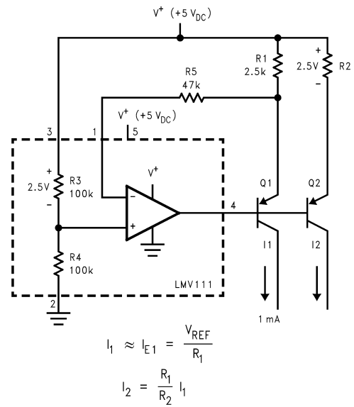
FIGURE 3. Fixed Current Source
