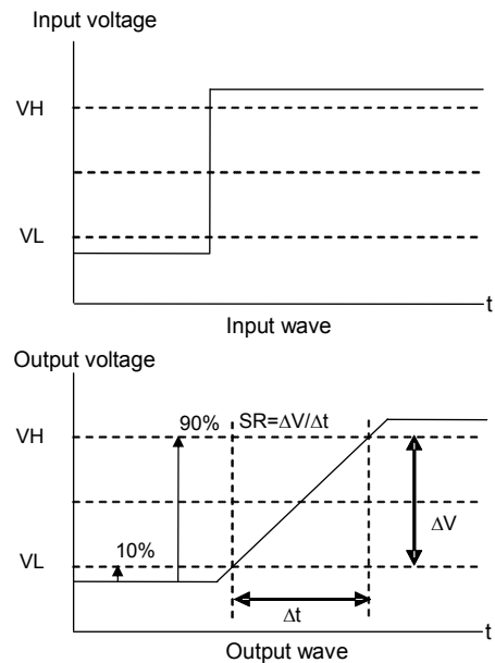
Figure 27. Slew Rate Input and Output Wave
