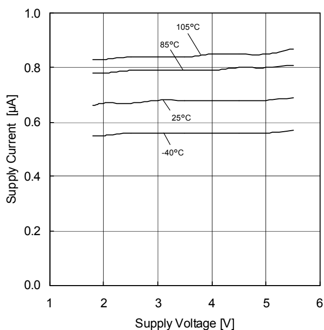
Figure 4. Supply Current vs Supply Voltage
