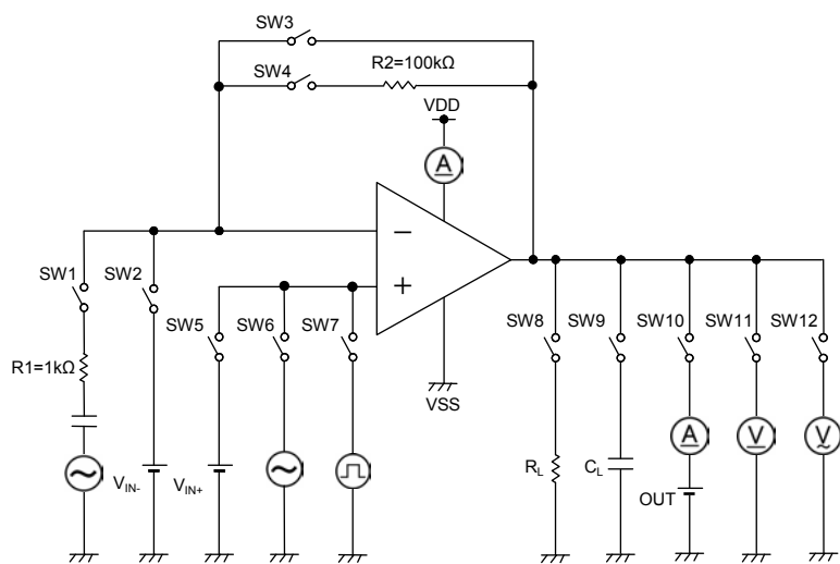
Figure 26. Test circuit 2
