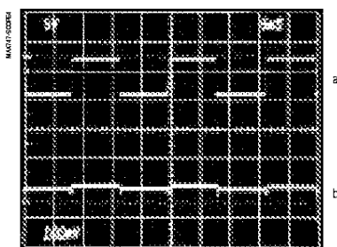
LINE-TRANSIENT RESPONSE
