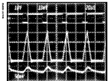
DISCONTINUOUS-CONDUCTION IDLE-MODE WAVEFORMS
