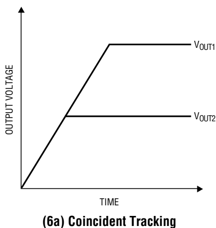
Figure 6. Two Different Forms of Output Voltage Sequencing
