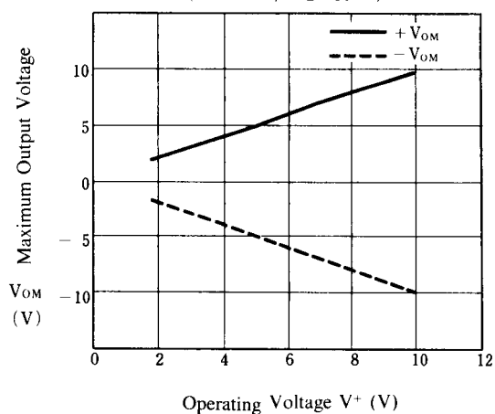
Maximum Output Voltage vs. Operating Voltage
