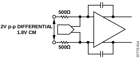
Figure 20. Equivalent Analog Input Circuit
