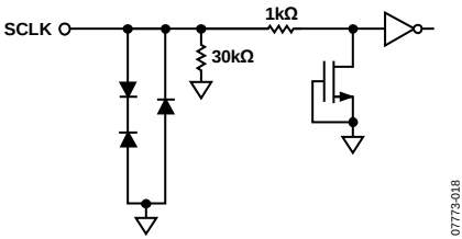
Figure 23. Equivalent SCLK Input Circuit
