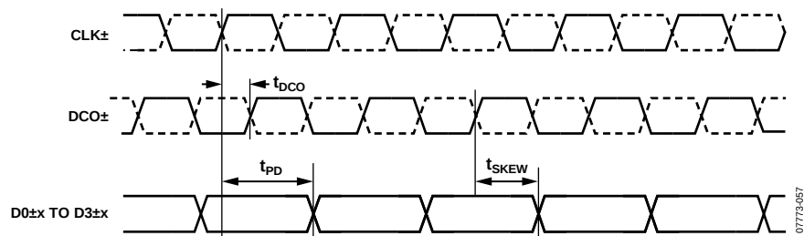
Figure 2. Timing Diagram
