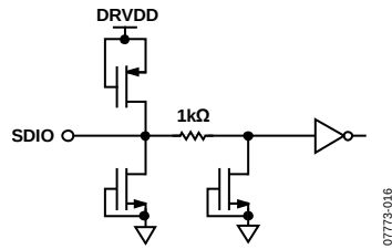
Figure 22. Equivalent SDIO Input Circuit
