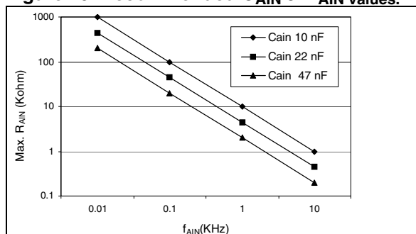
Figure 79. Recommended C_{AIN} & R_{AIN} values. 4)
