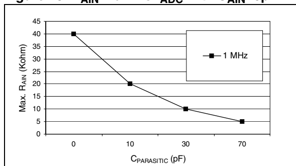
Figure 78. R_{AIN} max. vs f_{ADC} with C_{AIN}=0\text{pF} 3)
