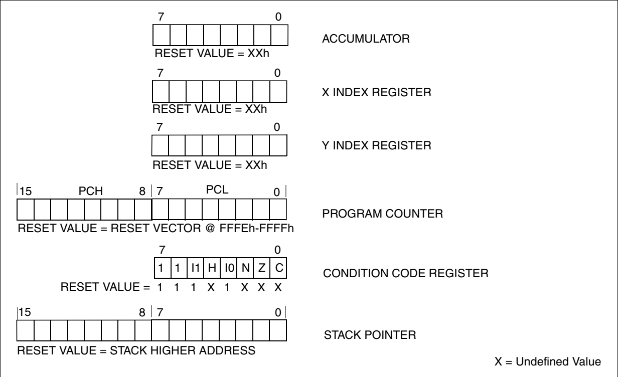
Figure 9. CPU Registers
