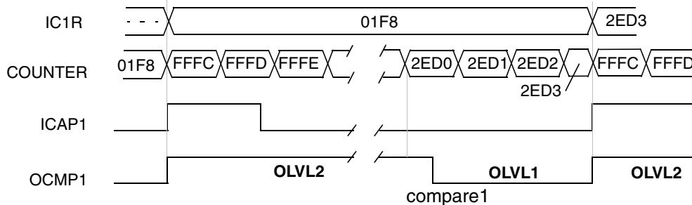
Figure 41. One Pulse Mode Timing Example
