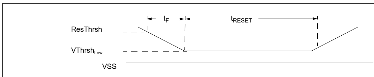
FIGURE 34-2: VTR RESET AND POWER-DOWN
