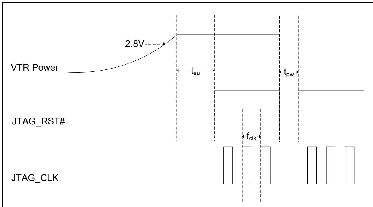
FIGURE 34-12: JTAG POWER-UP & ASYNCHRONOUS RESET TIMING
