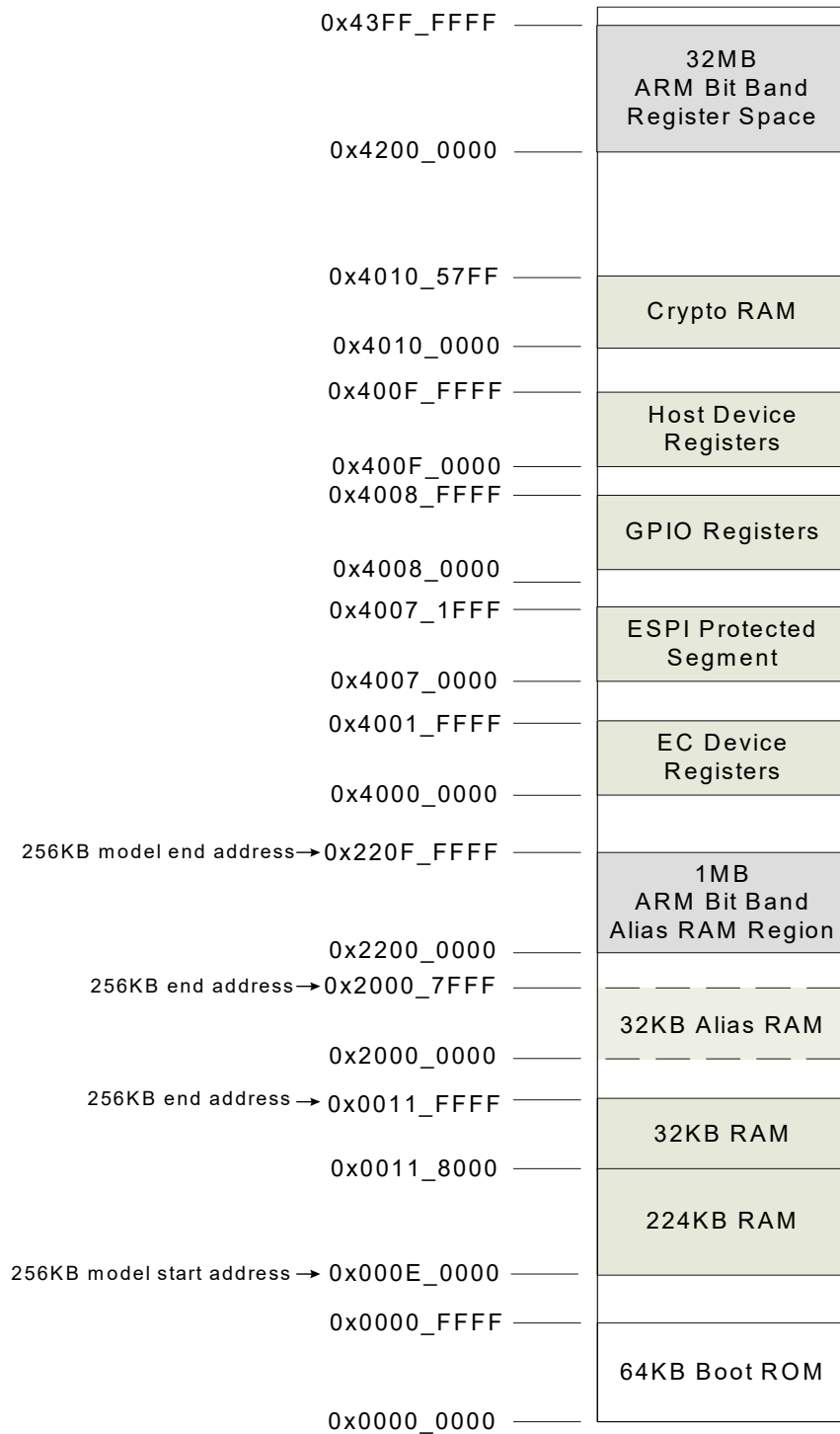
FIGURE 6-1: MEMORY LAYOUT
