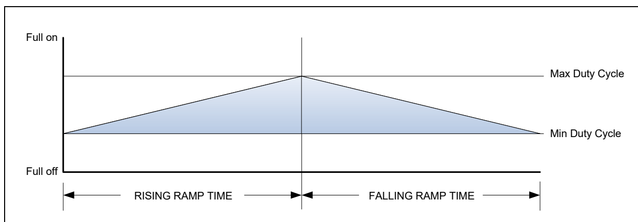
FIGURE 22-2: BREATHING LED EXAMPLE
