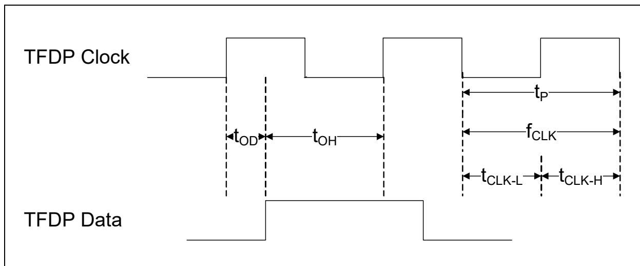
FIGURE 34-11: SERIAL DEBUG PORT TIMING PARAMETERS
