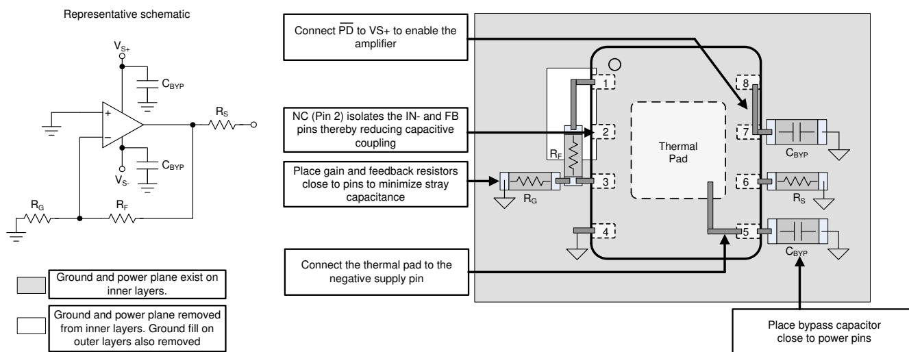
Figure 10-12. Layout Recommendation
