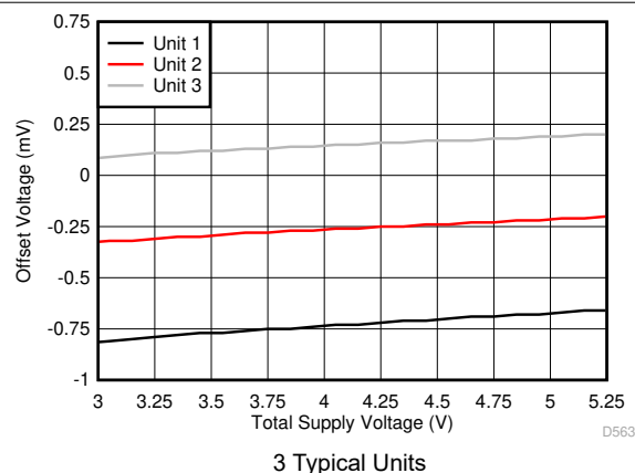
Figure 7-29. Offset Voltage vs Supply Voltage
