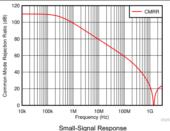
Figure 7-25. Common-Mode Rejection Ratio vs Frequency
