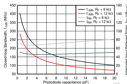
Photodiode Capacitance vs Bandwidth and Noise
