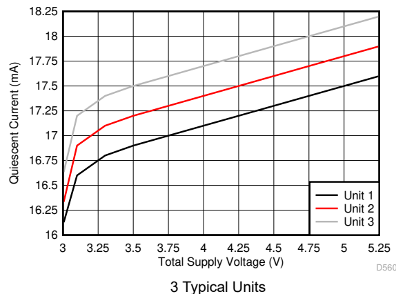
Figure 7-27. Quiescent Current vs Supply Voltage
