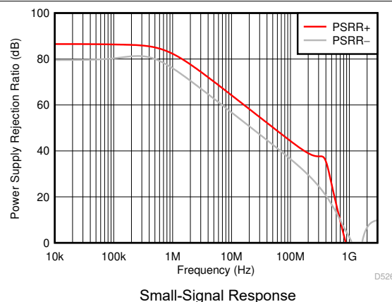
Figure 7-26. Power Supply Rejection Ratio vs Frequency
