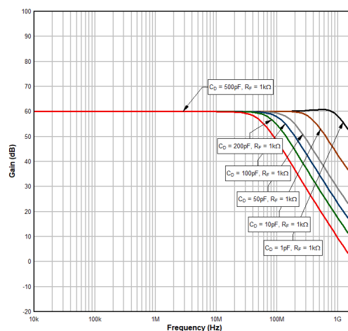
Figure 10-8. 1 Photodiode Input Characteristics TIA Frequency Response
