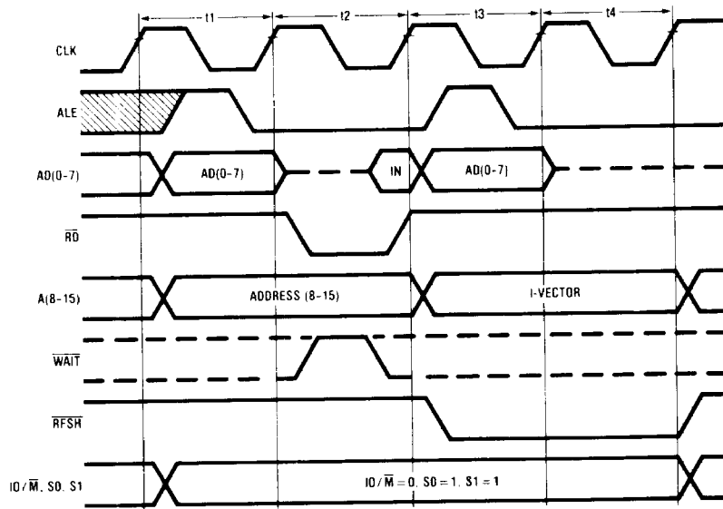
FIGURE 2a. Opcode Fetch Cycles without WAIT States
