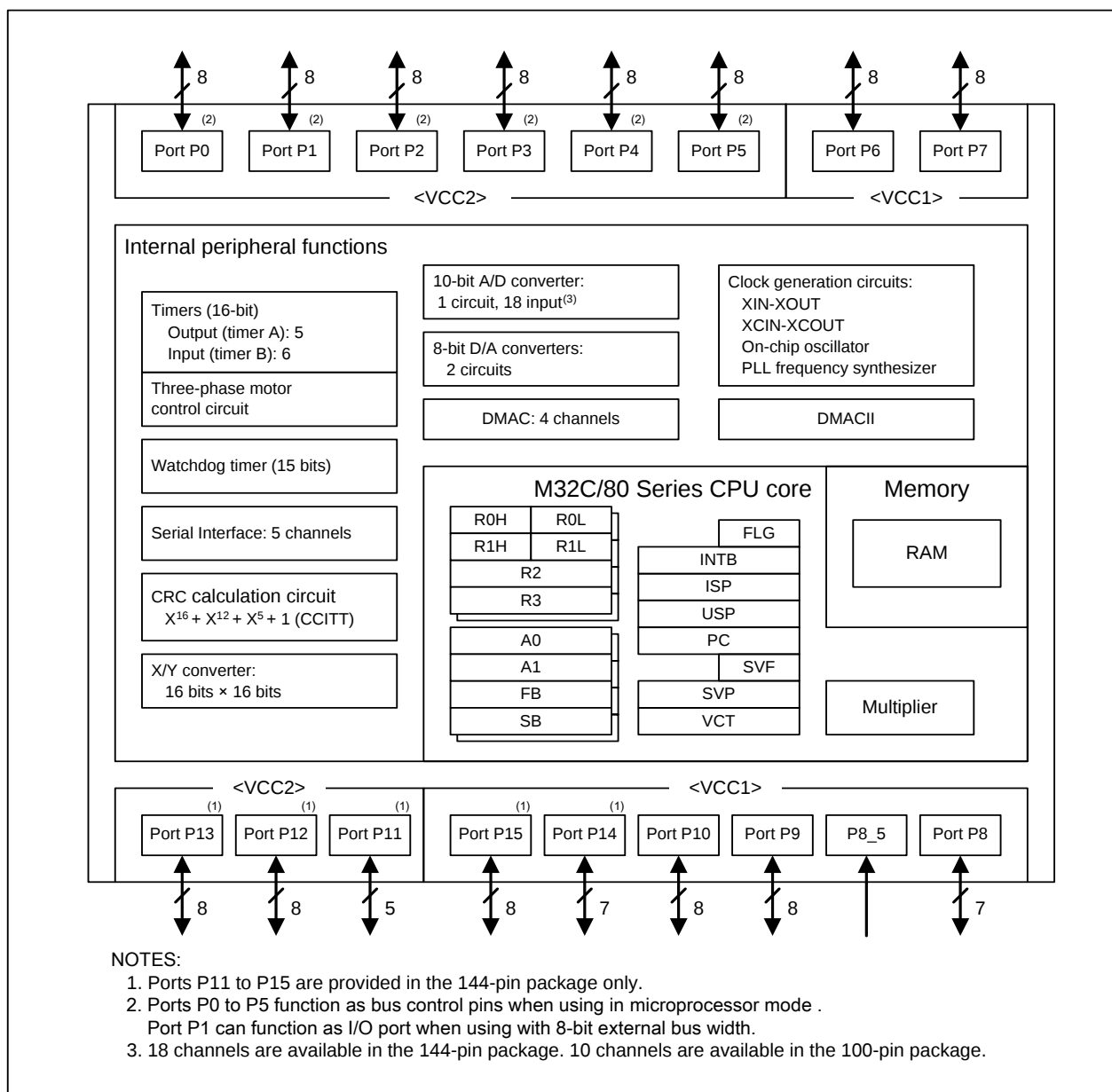
Figure 1.2 M32C/8A GroupM32C/8A Group Block Diagram
