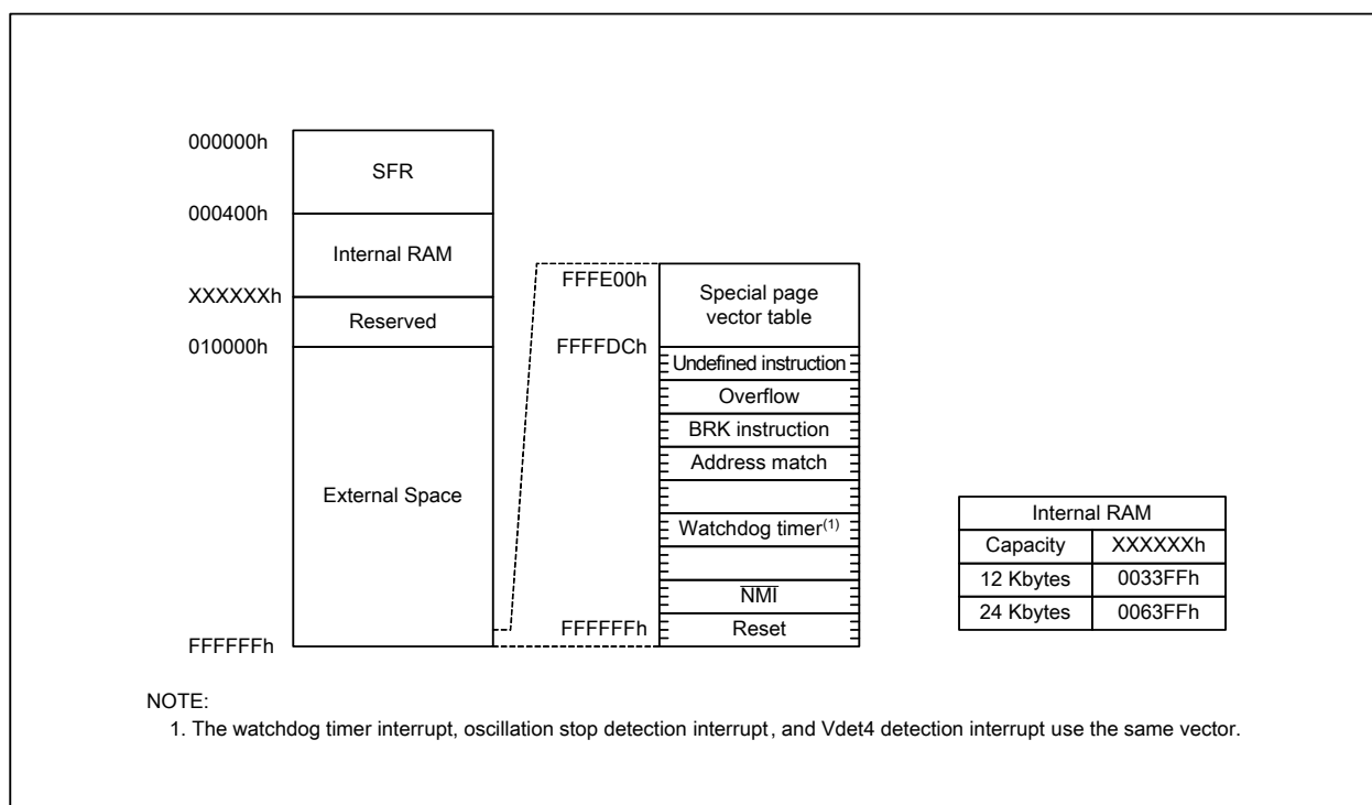
Figure 3.1 Memory Map
