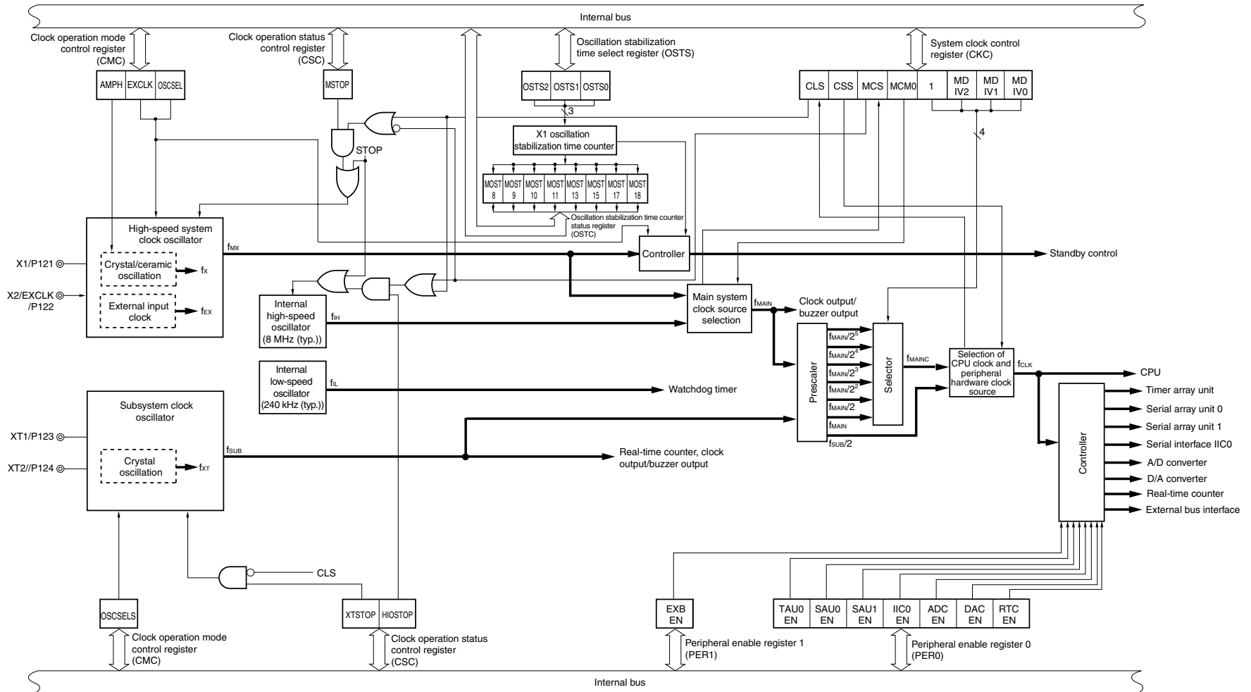
&lt;R&gt; Figure 6-1. Block Diagram of Clock Generator
