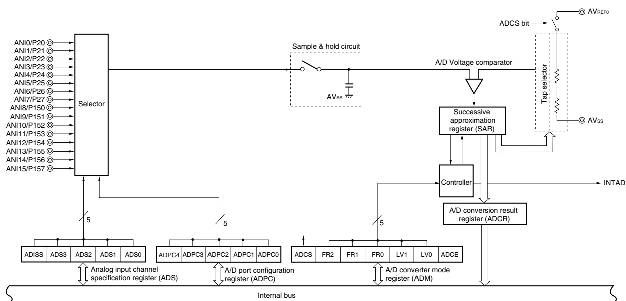
Figure 11-1. Block Diagram of A/D Converter
