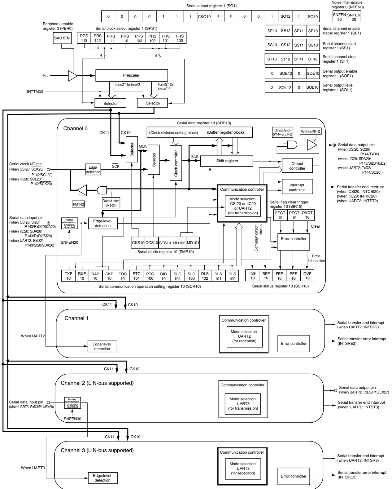
Figure 13-2. Block Diagram of Serial Array Unit 1
