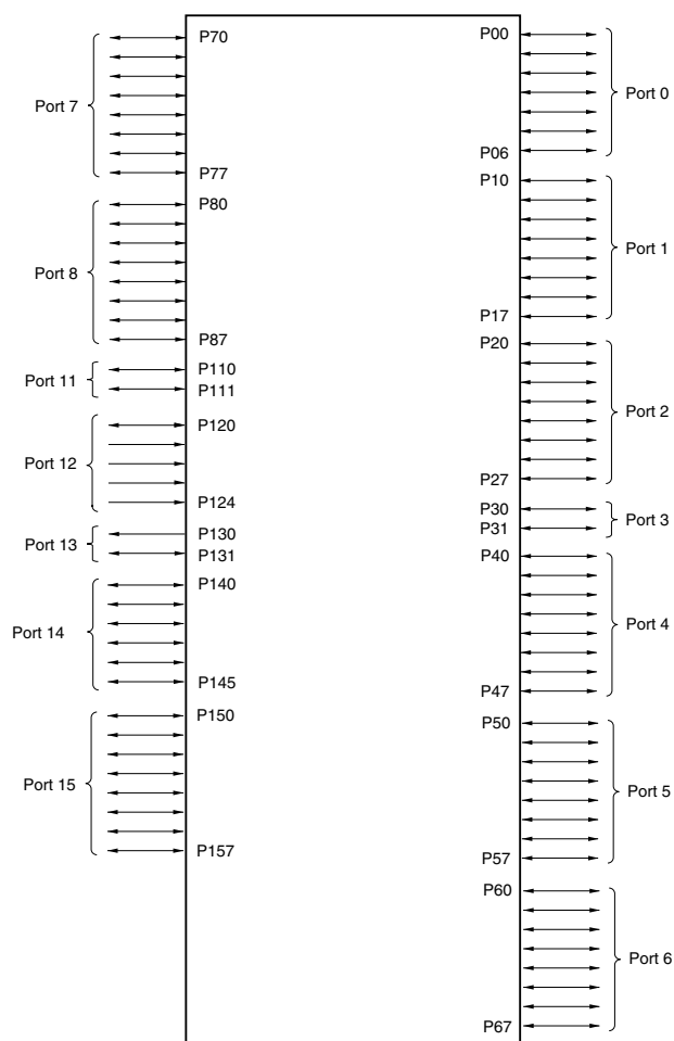
Figure 4-1. Port Types
