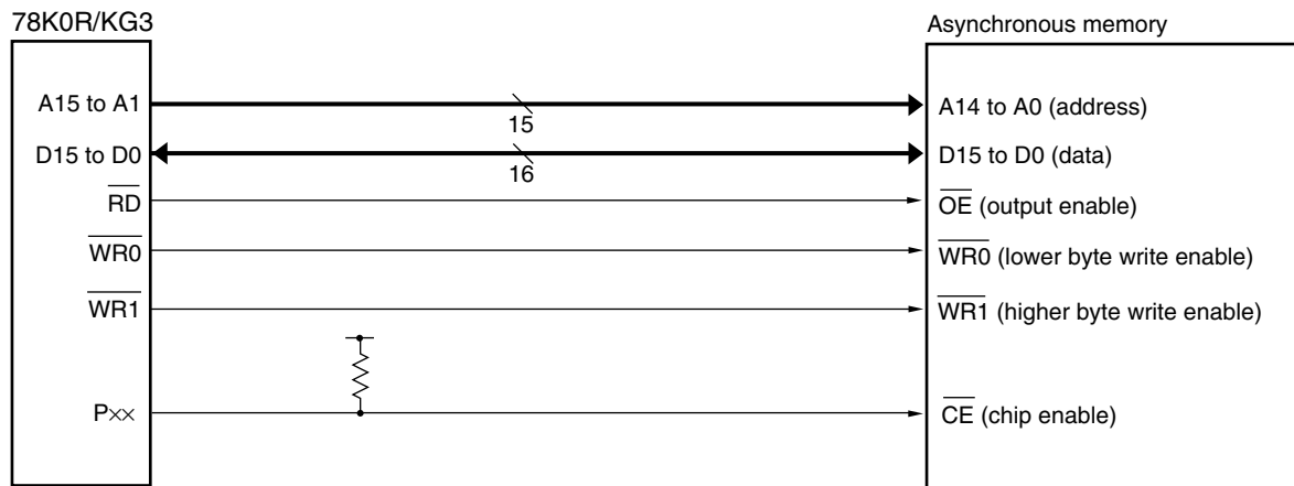
Figure 5-11. Example of Asynchronous Memory Connection
