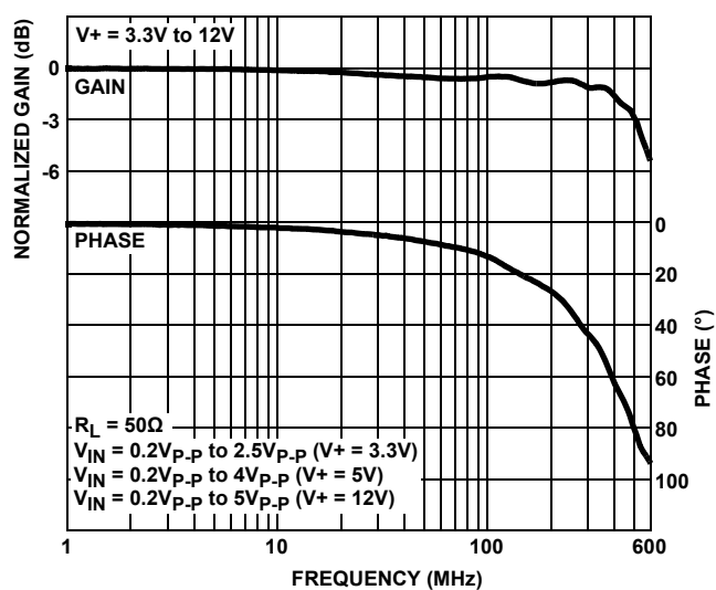
FIGURE 16. FREQUENCY RESPONSE
