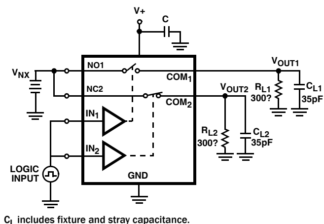
FIGURE 3B. TEST CIRCUIT (ISL5122 ONLY)
