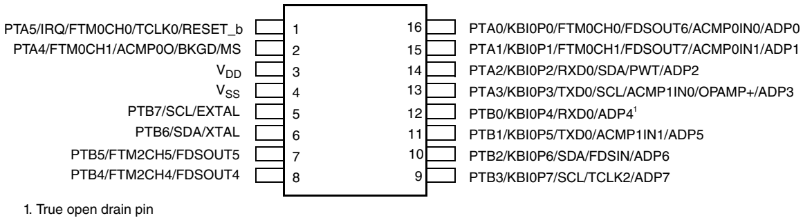
Figure 18. 16-pin TSSOP package
