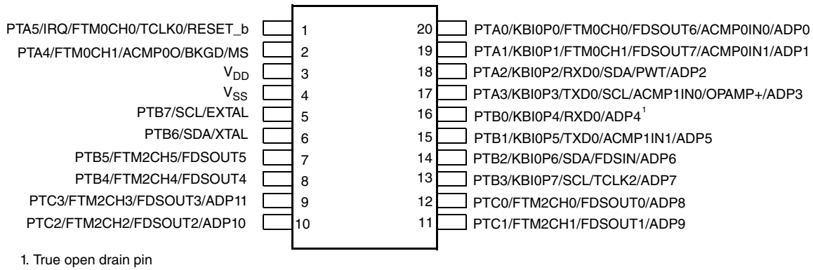
Figure 17. 20-pin TSSOP package
