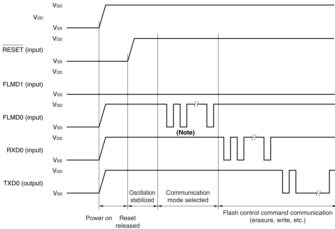
Figure 26-9. Selection of Communication Mode
