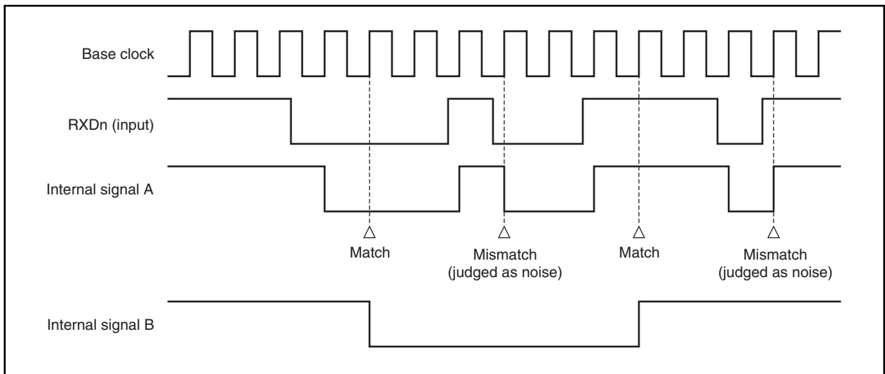
Figure 16-11. Timing of RXDn Signal Judged as Noise
