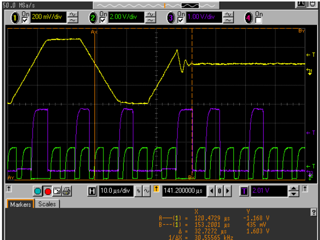
FIGURE 23. ENT BIT GOING LOW TO TONE DISABLED ON THE OUTPUT DELAY IS ~32μs
