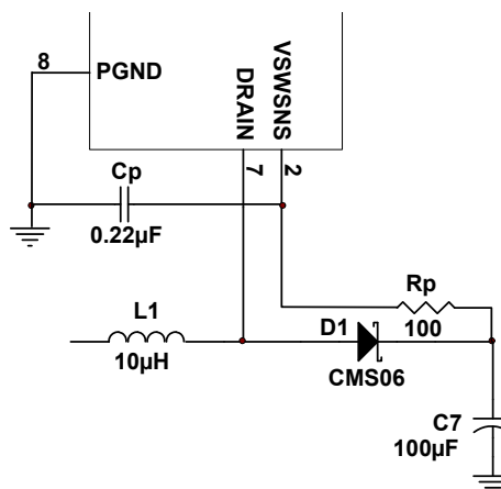
FIGURE 25. ADDITIONAL POLE ADDED BY R_p AND C_p TO COMPENSATE HIGH ESR ZERO
