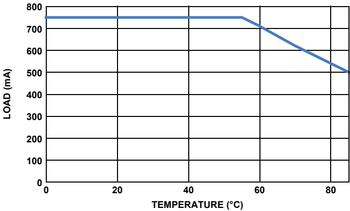
FIGURE 24. OUTPUT CURRENT DERATING
