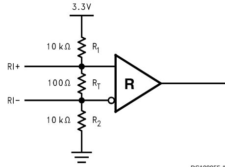
FIGURE 8. Terminated Input Failsafe Circuit
