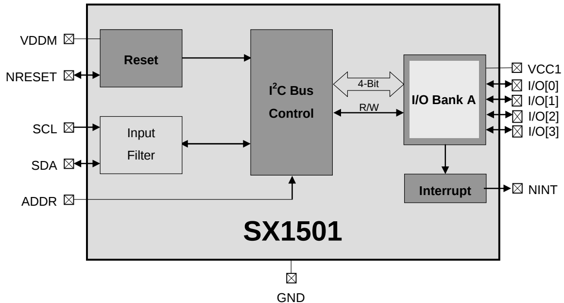
Figure 4 – 4-channel Low Voltage GPIO
