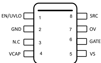
Figure 5-1. DDF Package 8-Pin SOT-23 LM74502, LM74502H Top View
