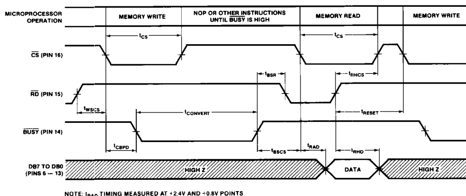
FIGURE 2: Static RAM Mode Timing Diagram
