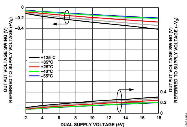
Figure 10. Output Voltage Swing Referred to Supply Voltage vs. Dual Supply Voltage, R_{LOAD} = 10 k\Omega , G = 10 , V_{REF} = 0 V
