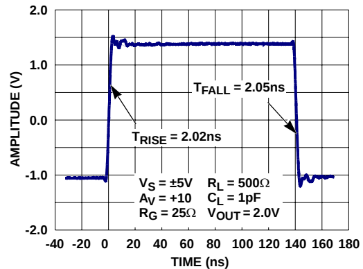
FIGURE 30. LARGE SIGNAL STEP RESPONSE_RISE AND FALL TIME
