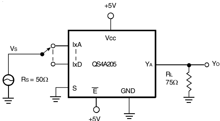
Off-Isolation
