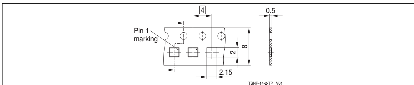
Figure 5-4 Tape (dimension in mm) for TSNP-14-2
