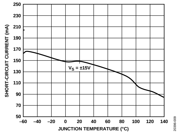
Figure 7. Short-Circuit Current vs. Junction Temperature
