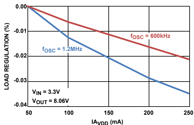
FIGURE 2. A_{VDD} LOAD REGULATION vs I_{A_{VDD}}
