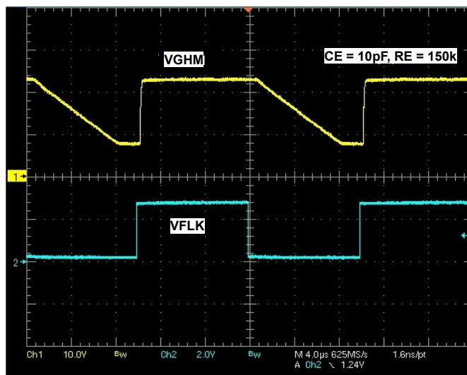
FIGURE 8. GPM CIRCUIT WAVEFORM
