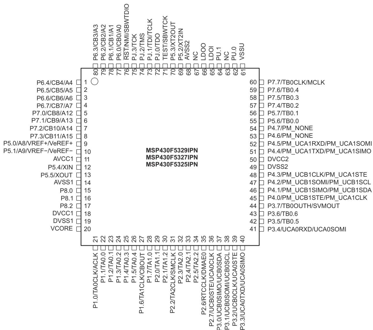
Figure 7-1. 80-Pin PN Package (Top View) – MSP430F5329IPN, MSP430F5327IPN, MSP430F5325IPN
