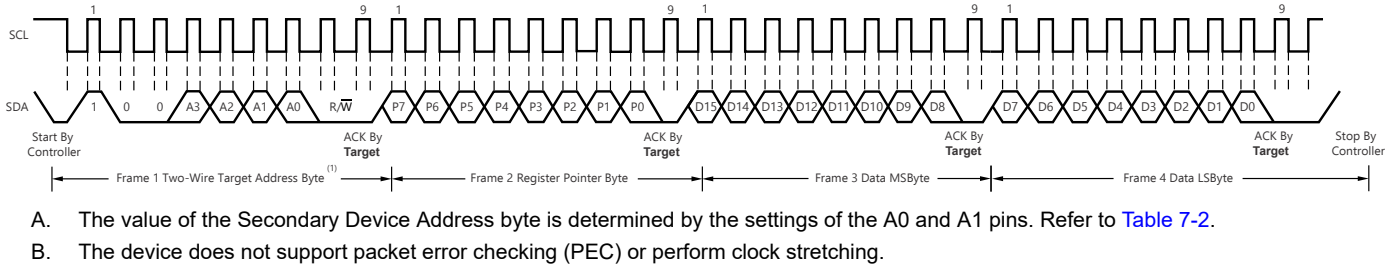
Figure 7-7. Timing Diagram for Write Word Format
