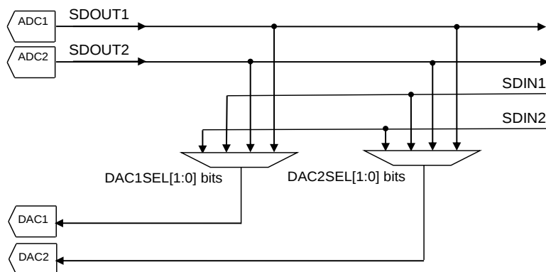
Figure 29. DAC1/2 source multiplexer
