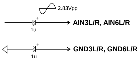
Figure 26. Pseudo-differential Input Mode (AD1LSEL[1:0] = AD1RSEL[1:0] = AD2LSEL[1:0] = AD2RSEL[1:0] = "11")
