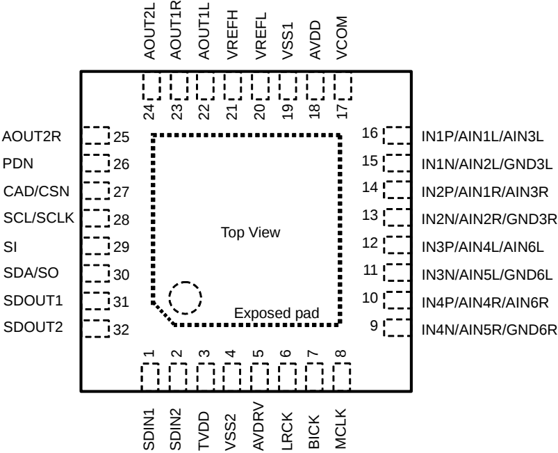
Figure 2. Pin Configuration
