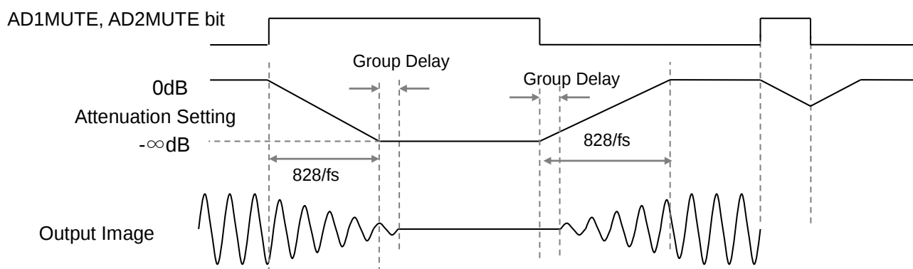
Figure 27. ADC Soft Mute
