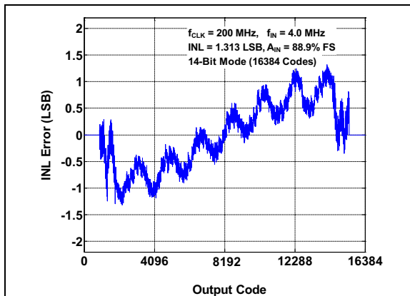
FIGURE 3-20: INL Error vs. Output Code: f_S = 200\text{ Msp} s, f_{IN} = 4\text{ MHz} .
