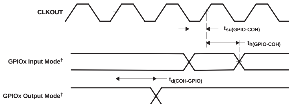
Figure 5-31. GPIOx Timings
