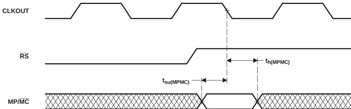
Figure 5-17. MP/MC Timing
