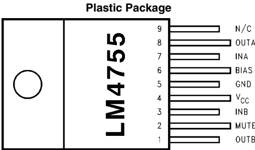
Package Description Top View Order Number LM4755T Package Number TA09A
