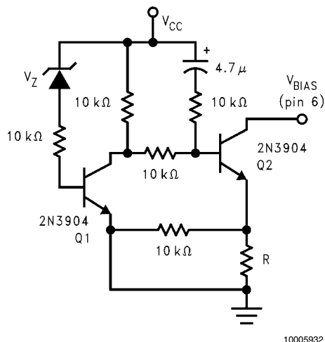
FIGURE 6. External Undervoltage Pull-Down
