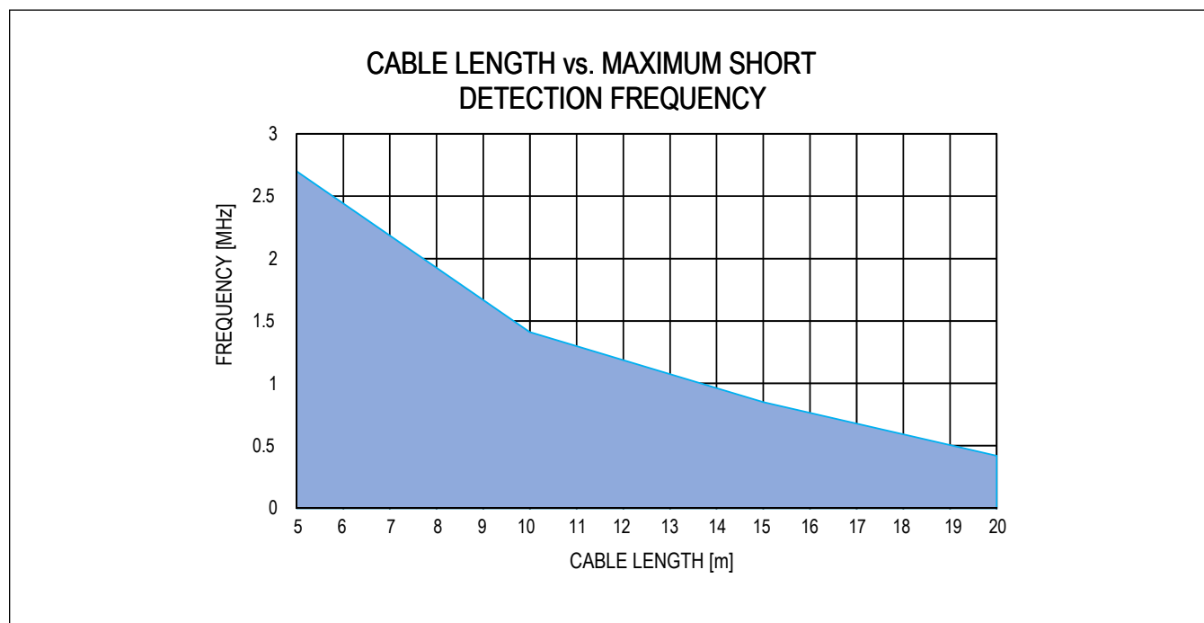
Figure 7. Overcurrent Detection Operating Frequency vs. Cable Length
