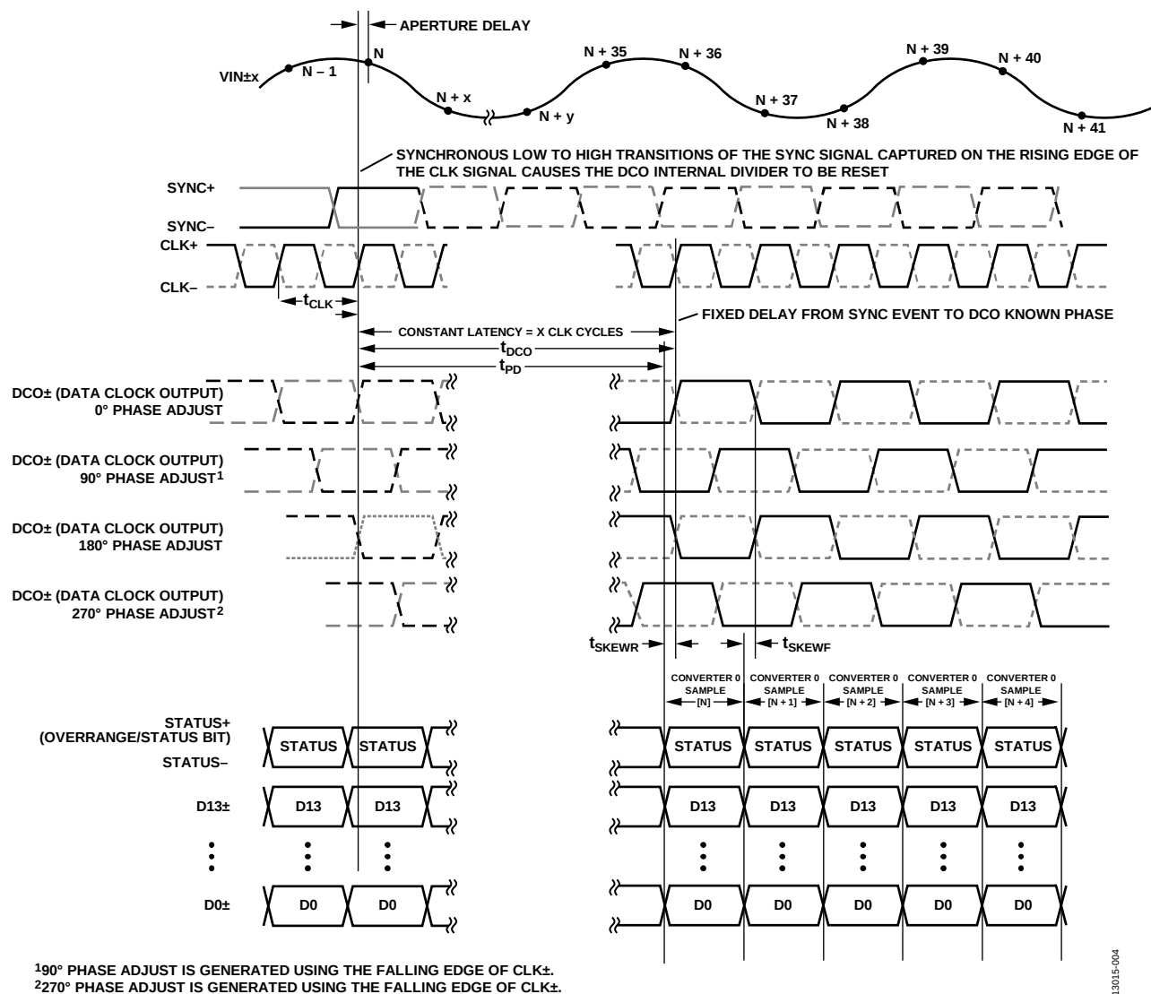
Figure 4. Parallel Interleaved Mode—One Converter, ≤14-Bit Data
