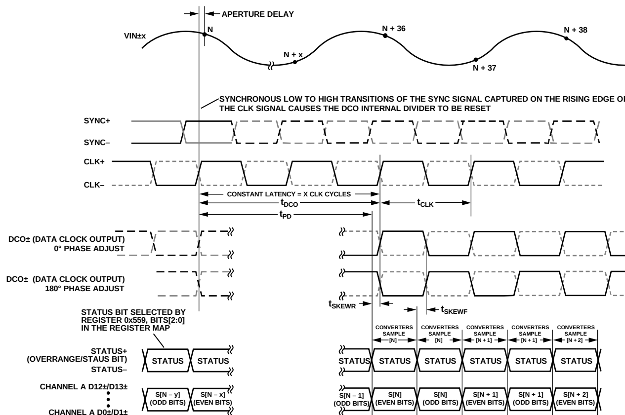
Figure 6. Channel Multiplexed (Even/Odd) Mode—One Converter, \leq 14 -Bit Data
