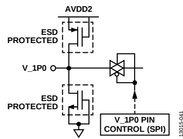
Figure 38. V_1P0 Input/Output
