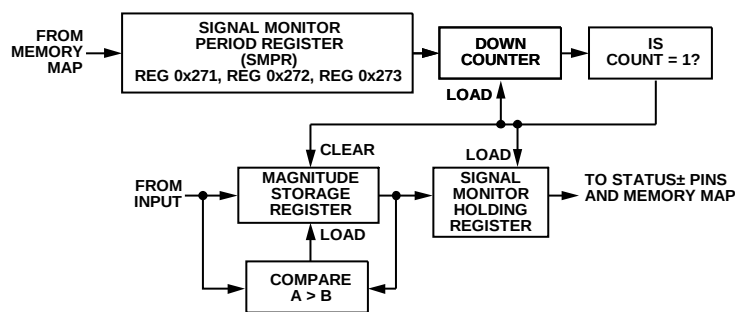
Figure 57. Signal Monitor Block
