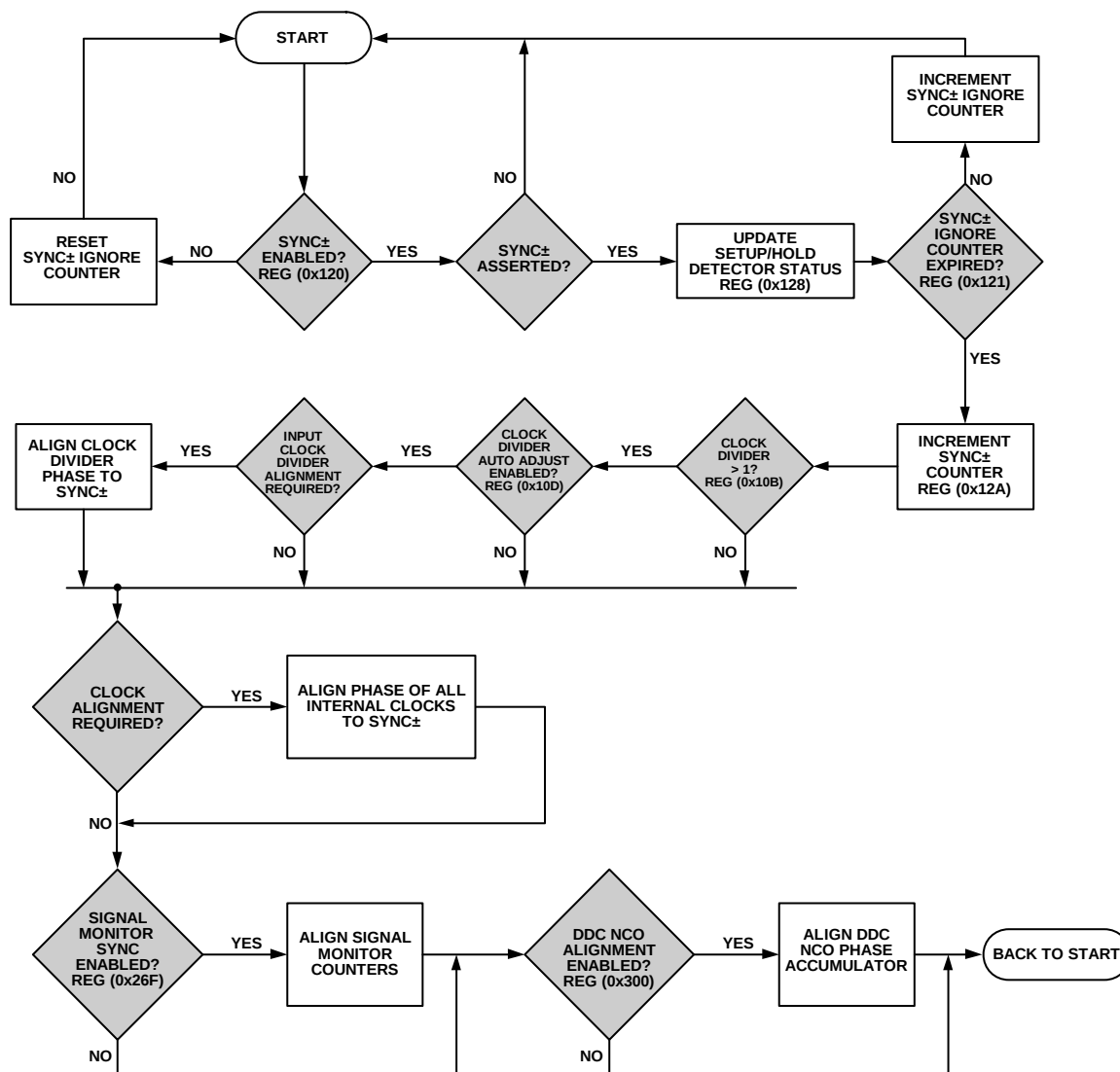
Figure 67. Multichip Synchronization
