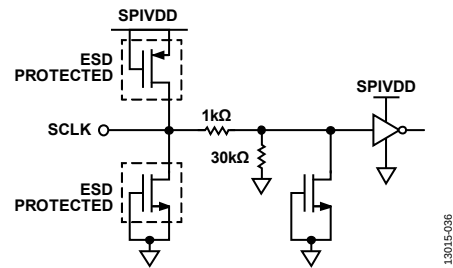
Figure 33. SCLK Inputs
