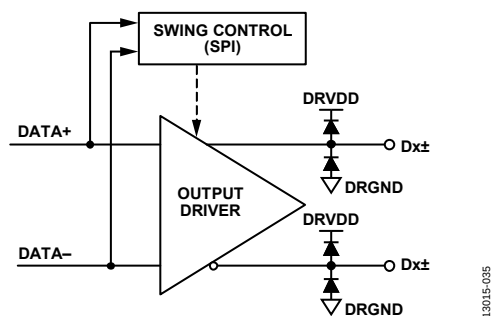
Figure 32. LVDS Digital Outputs, STATUS \pm , DCO \pm
