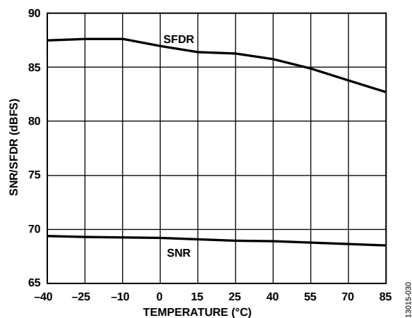
Figure 27. SNR/SFDR vs. Temperature, f_{IN} = 170.3 MHz
