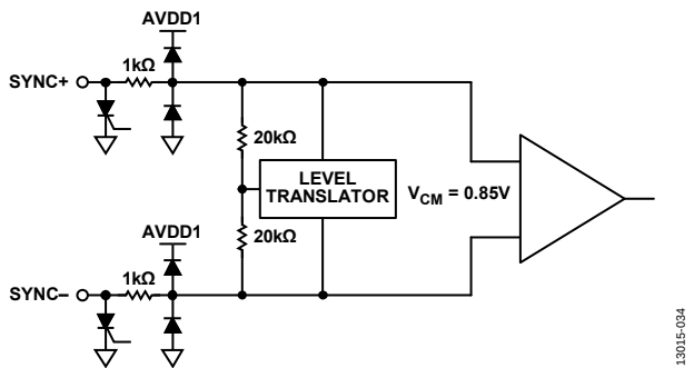
Figure 31. SYNC± Inputs
