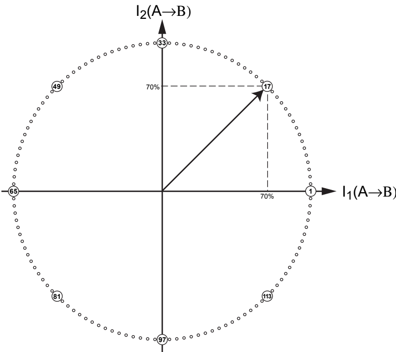
Figure 13: Thirty-Second Step MSX pins = 011. See Table 3 for step number detail
