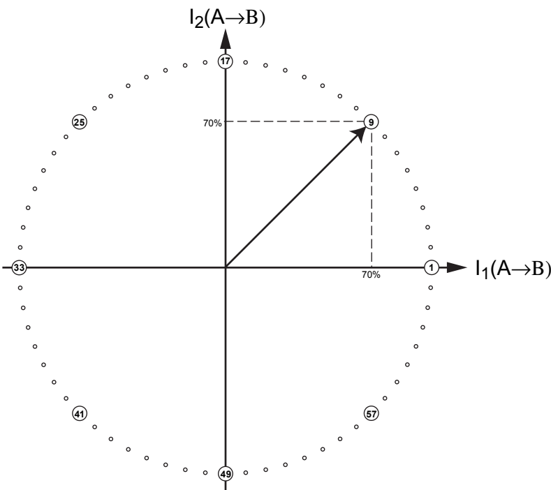
Figure 12: Sixteenth Step MSX pins = 010. See Table 3 for step number detail
