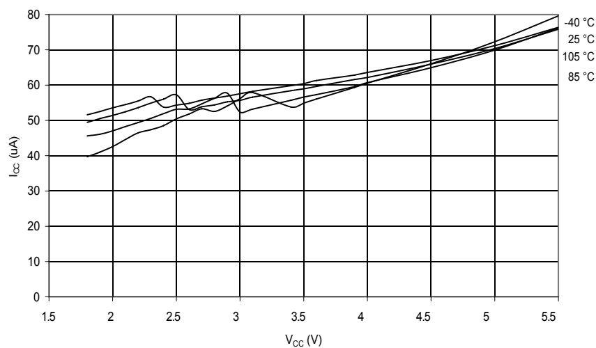
Figure 30-40. Analog Comparator Current vs. V_{CC}
