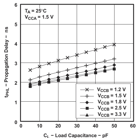
Figure 7-4. Typical Propagation Delay t_{PHL} (A to B) vs Load Capacitance
