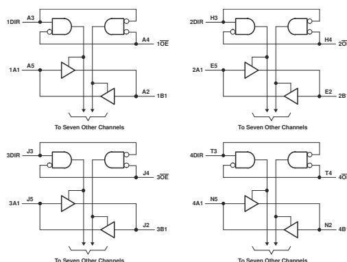
Figure 3-1. Logic Diagram
