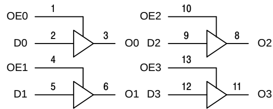
Figure 2. Logic Diagram
