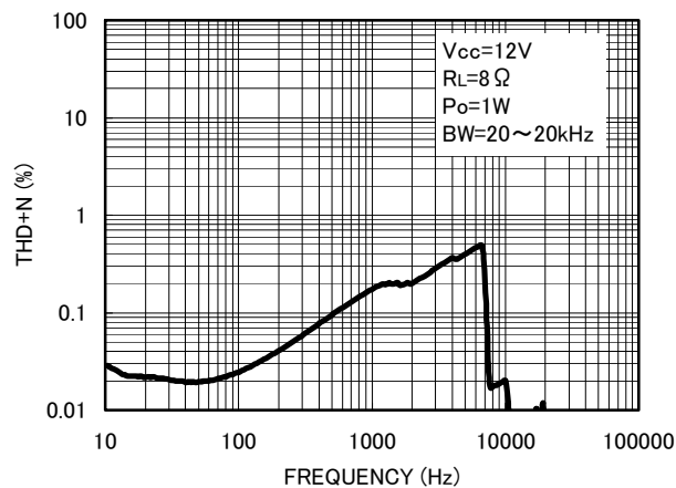
Fig. 2 THD+N — Frequency
