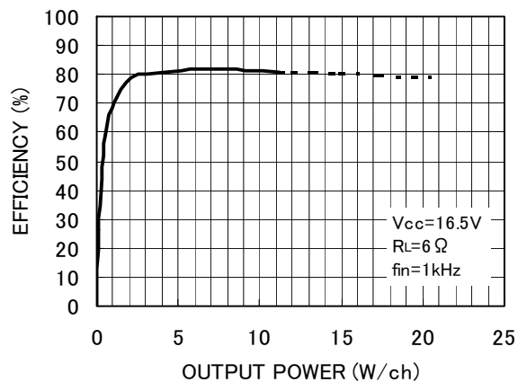
Fig. 21 Efficiency - Output power
