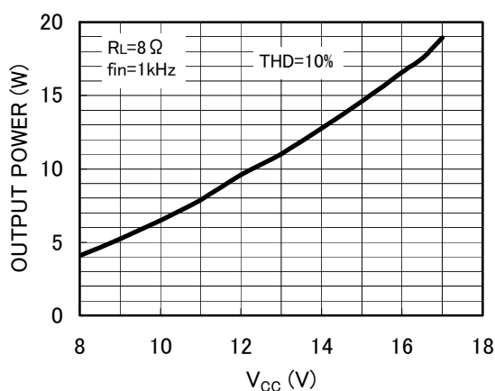
Fig. 6 Output power - Power supply voltage
