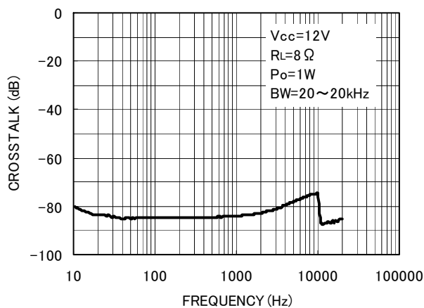
Fig. 4 Crosstalk - Frequency
