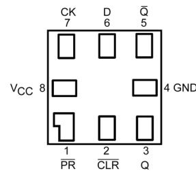
Figure 3. MicroPak™ (Top Through View)
