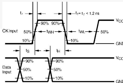
Figure 8. AC Waveforms
