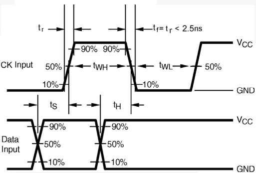
Figure 7. AC Waveforms
