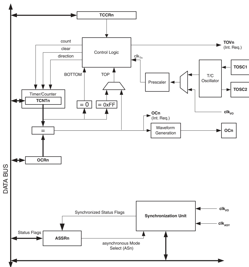
Figure 45. 8-bit Timer/Counter Block Diagram
