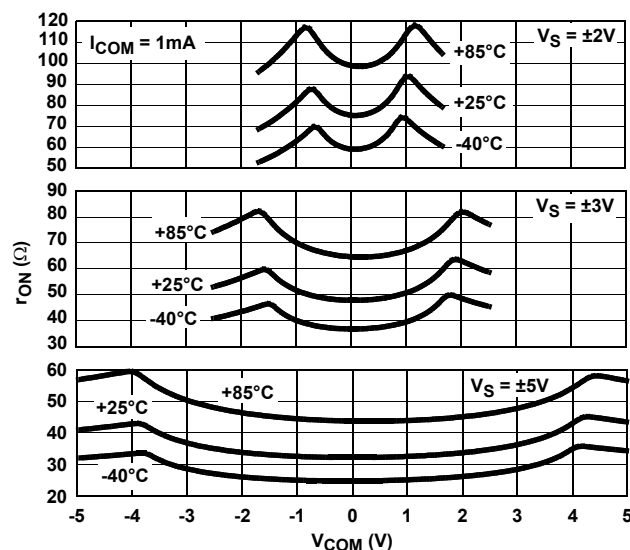
FIGURE 9. ON-RESISTANCE vs SWITCH VOLTAGE
