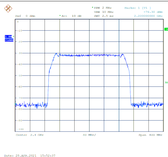
Figure 8-3. RF Signal at DAC Output
