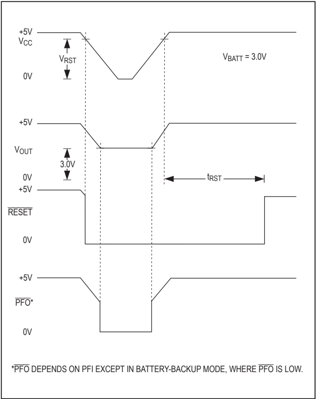
Figure 2. Timing Diagram
